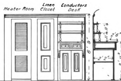
Fig. 486. Side Elevation of Conductor's Quarters.
