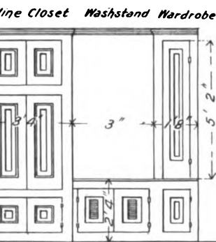
Fig. 485. Side Elevation of Conductor's Quarters.
