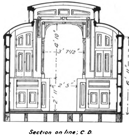
Fig. 481. Transverse Section showing Bulkhead.
