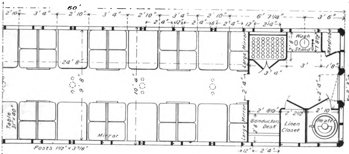
Fig. 482. Plan of Dining Room and Conductor's Quarters.
