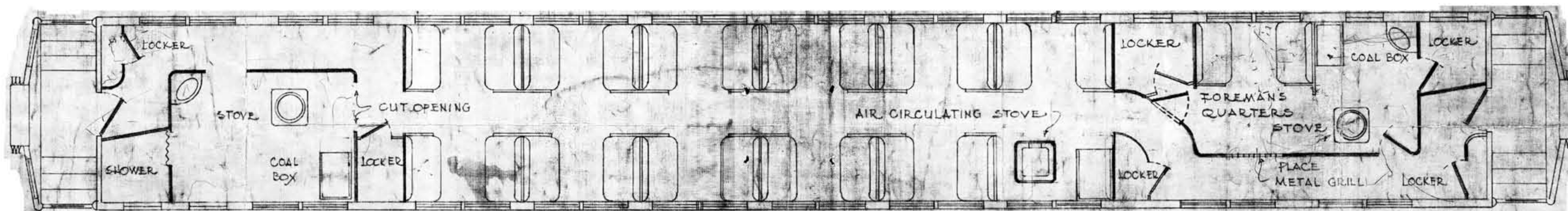
TOURIST SLEEPING CAR CONVERTED FOR USE AS SYSTEM GANG-BUNK CAR
